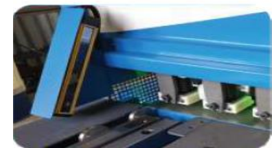
Finger protection with light guards (optional)
